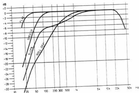
Filter – Frequenzkurven:
